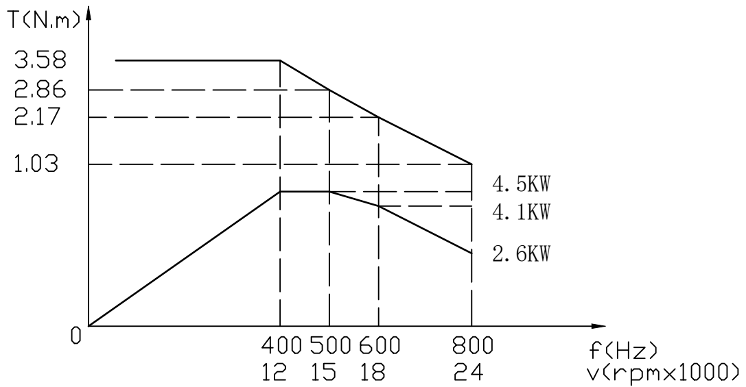
Torque/P.f Curve
